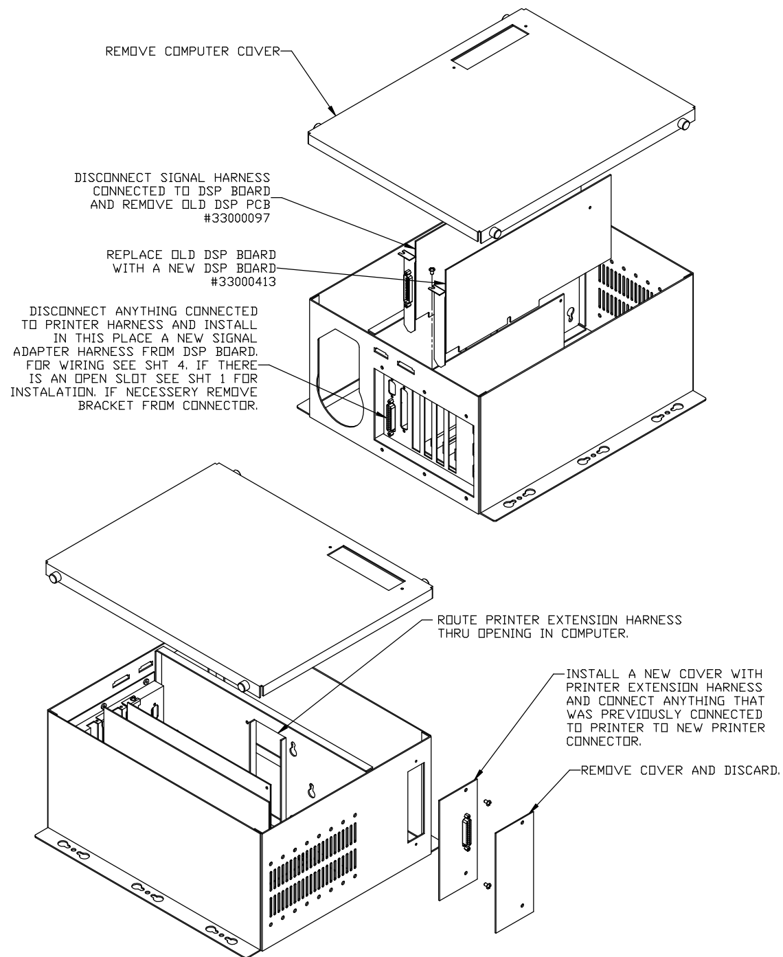
INSTALLATION OF REPLACEMENT DSP BOARD IN 4 SLOT BACKPLANE.
